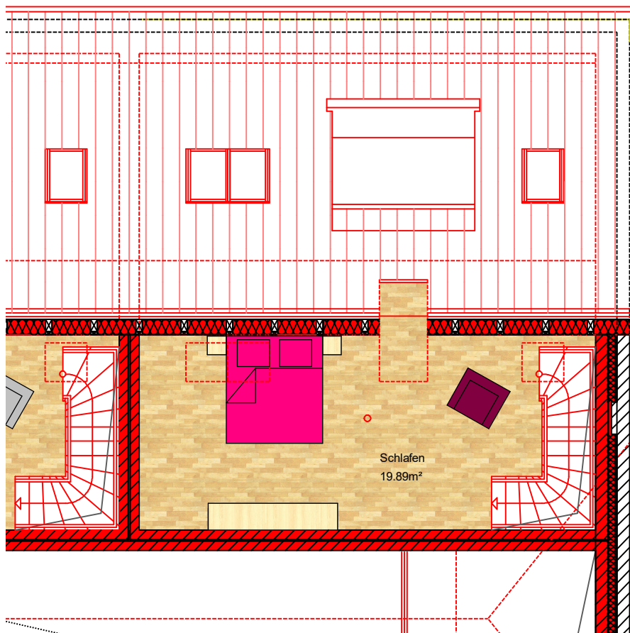
Grundriss WHG 8, 1:100
